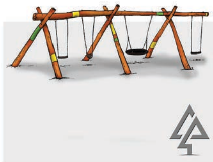
Triple A-Frame with Basket and Triple Swings 206-TAS
