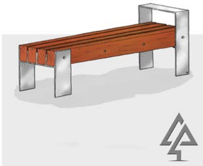
Bench Seat Type B with Armrest (807-BTA)
